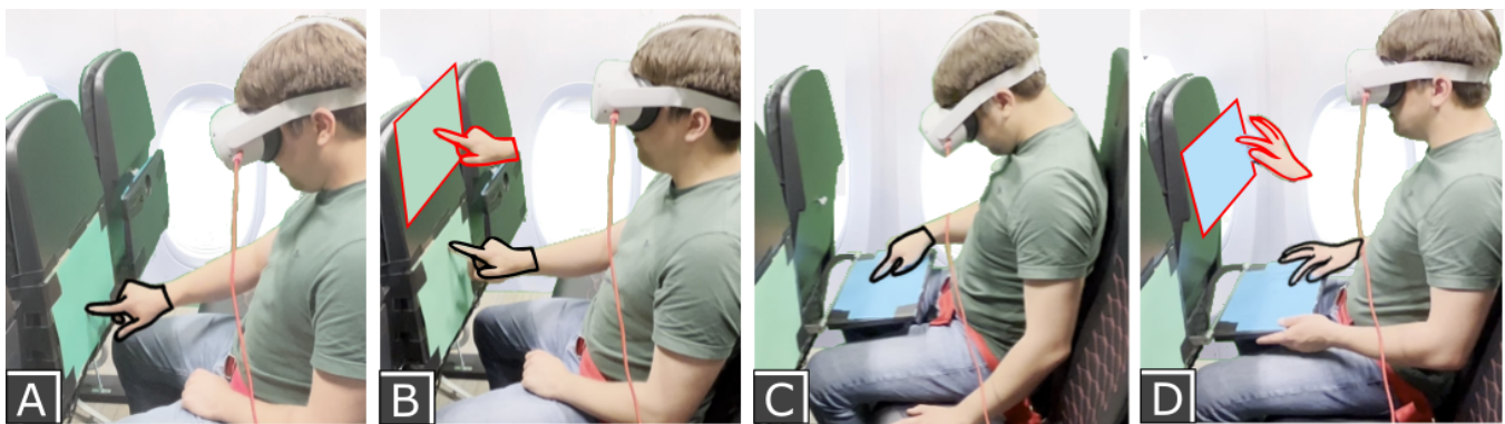
Figure 1: Using passive haptics surfaces in planes for interaction. (A) shows how the seat-back in front can be used as a passive haptic surface; (B) using translation remapping to create a more comfortable experience; (C) shows the use of a horizontal tray table for passive haptic input; and (D) using translational and rotational remapping for a more comfortable interaction.
